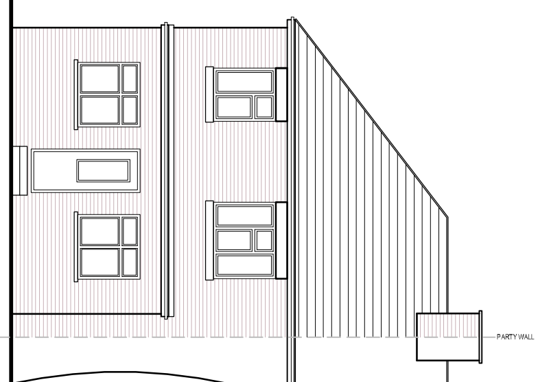
EXISTING REAR FACING EAST ELEVATION
